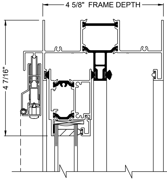
③ FIXED HEAD
